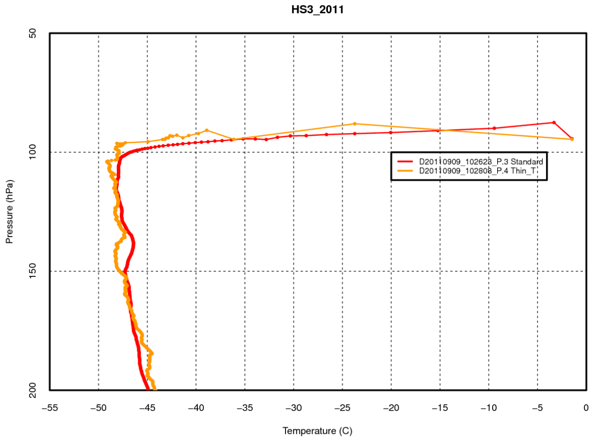
Figure 5 - Comparison between thin and standard temperature sensors
