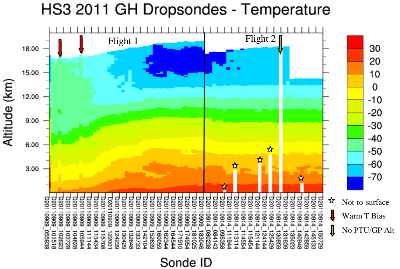
Figure 3- Temperature ( °C) profiles of final QCed data for all 79 soundings
