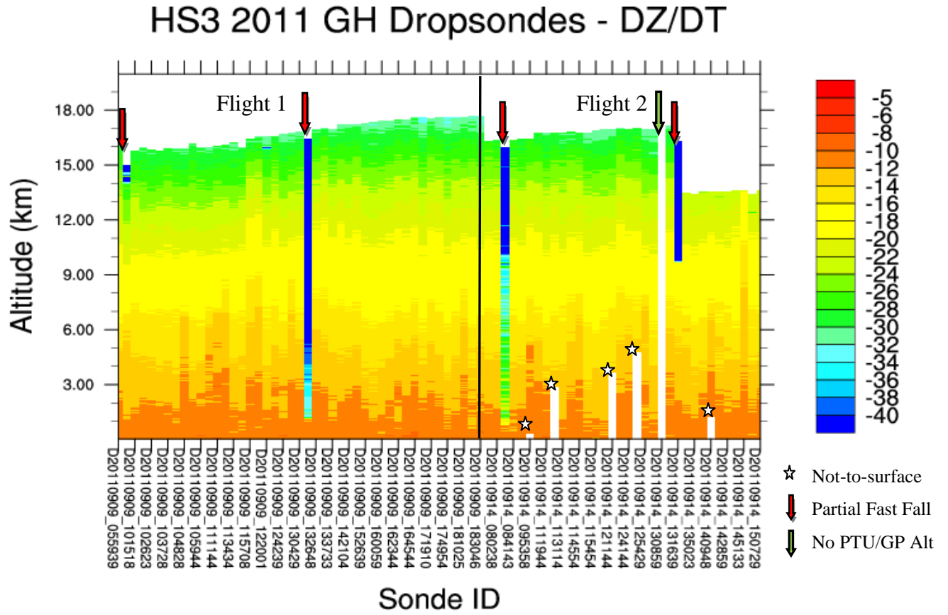
Figure 4 - Pressure-calculated fall rate (m/s) profiles of final QCed data for all 79 soundings
