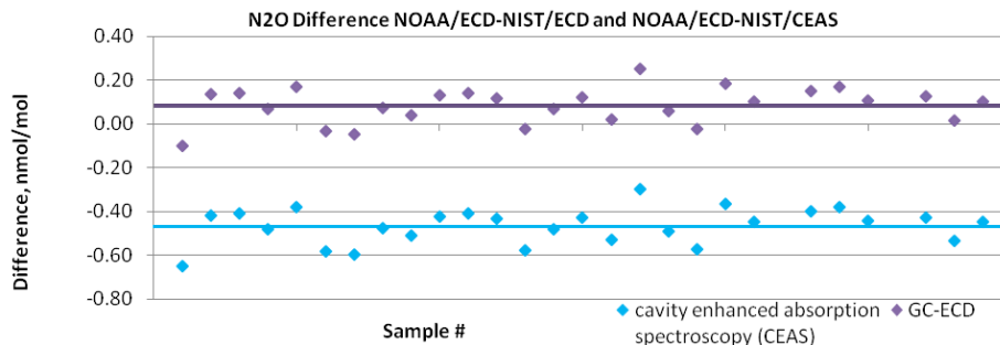
Figure 2. N 2 O difference NOAA/ECD-NIST/ECD and NOAA/ECD-NIST/CEAS.
