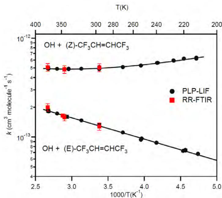
Figure 1. The temperature dependence of the rate coefficients measured for the OH reaction with ( E )- and ( Z )- CF 3 CH=CHCF 3 . PLP-LIF: Pulsed Laser Photolysis – Laser Induced Fluorescence; RR-FTIR: Relative Rate technique combined with Fourier transform infrared detection.
