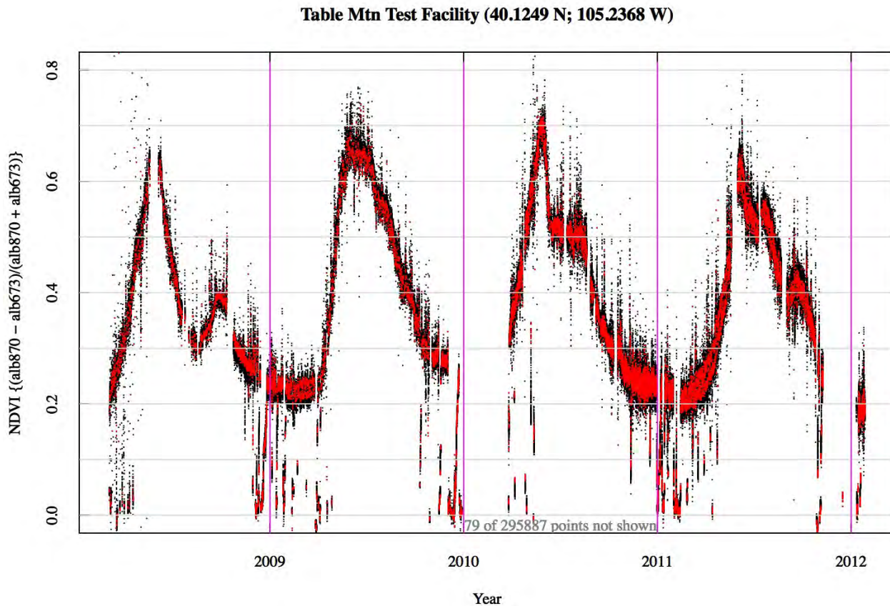
Figure 1. The normalized difference vegetative index for Table Mountain, 16 km north of Boulder, Colorado. Note the steep increase with a consistent peak in late May with a minimum in mid winter. After the May peak the path toward the winter minimum depends primarily on precipitation, and has a different character in each of the four years of this measurement history.
