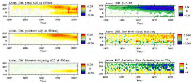
Figure 1. Latitude-time sections of zonal mean anomalies (total Aerosol Optical Depth, cloud effective radius, low level cloud fraction, net radiative flux perturbation) from 1900 to 2005.
