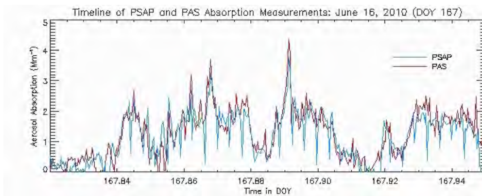
Figure 1. Timeline for the PSAP and PAS absorption measurements for June 16, 2010 (DOY 167) during a research flight on the CalNex field campaign. The flight depicted in figure 1 was where substantial time was spent flying over the agricultural fields of the San Joaquin Valley, over the cities of Fresno and Bakersfield, as well as over the Pacific ocean. It is clear that the \sigma_{ap} from both instruments follow closely in measure and magnitude, which was typical for all of the CalNex campaign.
