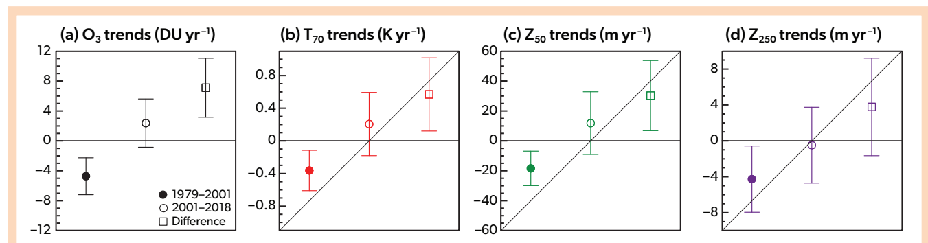
Figure 5-15. Trends in Southern Hemisphere high-latitude (65–90°S) ozone and circulation. (a) November ozone (DU yr -1 ), (b) November–December 70 hPa temperature (K yr -1 ), (c) November–December 50 hPa geopotential height (m yr -1 ), and (d) December–January 250 hPa geopotential height (m yr -1 ) for 1979–2001 (filled circles), 2001–2018 (open circles), and the difference (squares). Error bars represent the adjusted 95% confidence intervals of the trends. Ozone data are from the TOMS/OMI merged ozone dataset; temperature and geopotential height are from ERA5. [From Zambri et al., 2021.]
