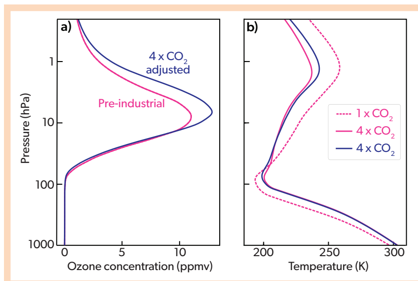
Figure 5-10. Stratospheric ozone feedback on temperature changes simulated by a simple 1-D radiative convective equilibrium model. Vertical profile of (left) tropical mean zonal mean ozone for preindustrial climate (pink) and for 4xCO 2 (blue), and (right) resulting temperature profiles from the model for preindustrial climate (pink dashed), and for 4xCO 2 forcing when prescribing the preindustrial ozone profile (pink) or the 4xCO 2 ozone profile (blue). [Adapted from Dacie et al., 2019.]
