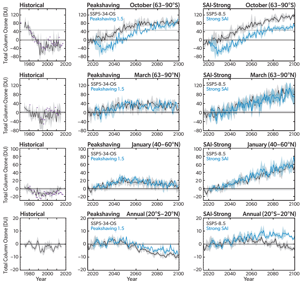
Figure 6-13. Simulated impacts on TCO in different latitude bands and seasons (rows), relative to the 2015–2025 TCO average, for the past (historical; left column) and projected for the peakshaving (middle column) and strong (right column) SAI scenarios. The ensemble means are shown for the baseline scenario (black) with standard deviation (gray shading) and for the SAI experiments (blue) with the standard deviation (light blue shading) based on simulations with CESM2(WACCM6) using SSP5-3.4-OS and SSP5-8.5 for the baseline scenarios, against which the peakshaving and strong SAI scenarios are compared, respectively. Black horizontal lines indicate the 2020 values and gray lines the 1980 values, based on the model simulations. In the historical TCO panels, a three-year running mean has been applied to the TCO observations from the Solar Backscatter Ultraviolet (SBUV) Merged Ozone Data Set (Frith et al., 2017; purple symbols) to facilitate comparison with the ensemble mean of the control simulation.
