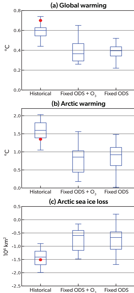
Figure 5-9. Climate impact of ODSs for the period 1955–2005. (a) Annual mean global surface-temperature change over the period 1955–2005 for each ten-member Community Earth System Model Version 1 (CESM-CAM5) ensemble, as labelled on the abscissa. The boxes extend from the lower to upper quartile of the data, with a line at the median and whiskers showing the entire range across each ensemble (b) As in (a) but for Arctic temperatures, averaged (60–90°N). (c) As in (a) but for September Arctic sea ice extent. Red circles denote the observed values obtained from GISTEMP27 v.3 for surface temperature and HadISST28v.2.2.0 for sea ice. The change over the period 1955–2005 is computed as the linear trend multiplied by the number of years (51). In each panel, the means of the Fixed ODS and ozone (Fixed ODS+O 3 ) (ODSs and stratospheric ozone fixed at year 1955 levels) and Fixed ODS (ODSs fixed at year 1955 levels) ensembles are significantly different from that of the Historical ensemble at the 99% confidence level by two-tailed t-test. [Adapted from Polvani et al., 2020.]
