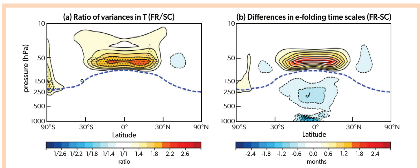
Figure 5-13. Impact of ozone variations on temperature variability. (a) Ratio of zonal mean temperature variance between a WACCM simulation with interactive ozone (FR) and one with specified ozone (SC), and (b) the difference in the e-folding timescale of temperature (in months) between the two simulations (FR-SC). [Adapted from Yook et al., 2020.]
