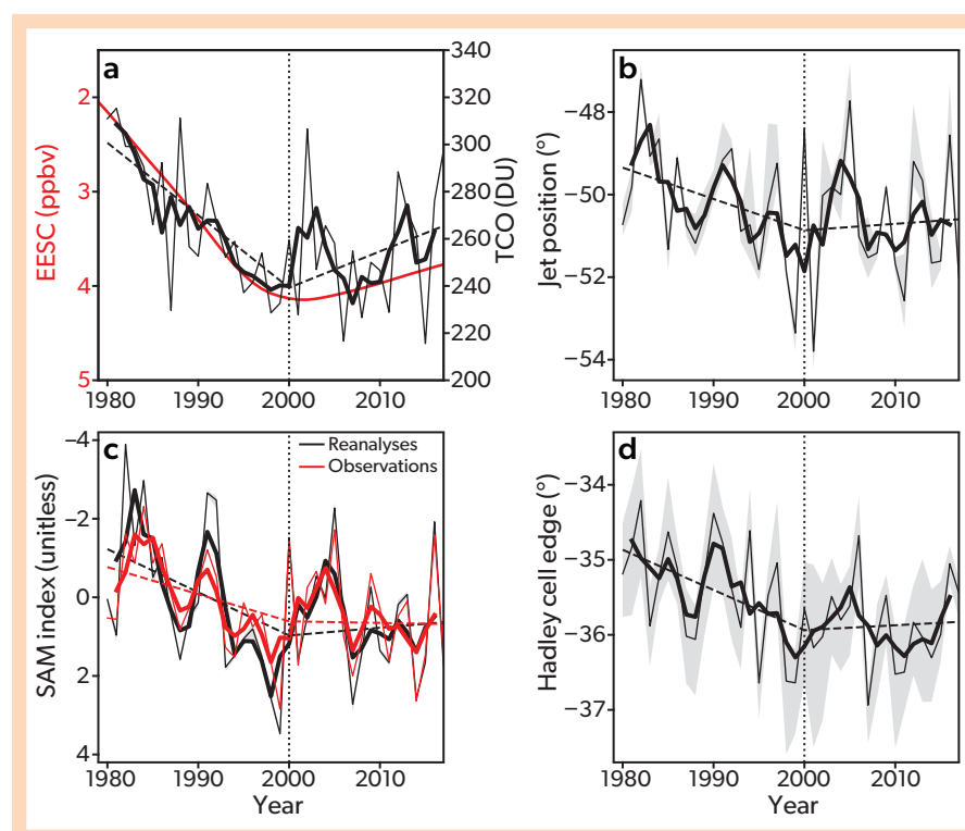
Figure 5-14. Observed total ozone and Southern Hemisphere tropospheric circulation. Time series of (a) EESC (note the inverted left y axis) for polar winter conditions and Antarctic total column ozone (TCO; right axis) averaged over September through November, with the latter measured by SBUV (in DU). (b) position of the SH mid-latitude jet in reanalysis data in DJF, (c) the SAM index (note the inverted y axis) as derived from reanalysis data and from station observations in DJF, (d) position of the edge of the Hadley cell in reanalysis data in DJF. Reanalysis data are averages across four products (ERA-I, JRA-55, MERRA2-ana and MERRA2-asm). The thin lines are unsmoothed quantities, and thick lines represent centered three-year smoothed values. Two piecewise continuous linear trend lines for the unsmoothed data (dashed lines) are drawn for the periods 1980–2000 and 2000–2017. [From Banerjee et al., 2020.]
