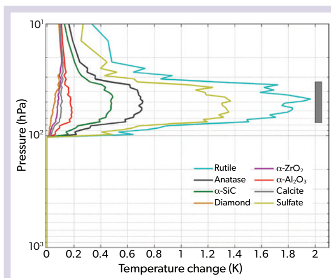
Figure 6-17. Equilibrium stratospheric heating produced by a mass of monodisperse solid aerosols of optimized radii sufficient to achieve -1 \text{ Wm}^{-2} shortwave radiative forcing. The gray bar on the right shows the approximate location of the aerosol layer. [Adapted from Dykema et al., 2016.]
