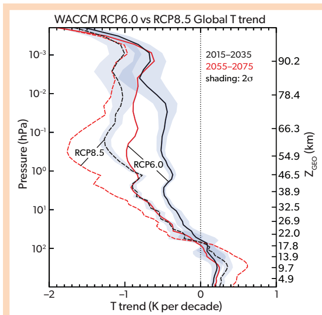
Figure 5-2. Projected global mean temperature trend profiles for periods in the early (2015–2035) and late (2055–2075) 21 st century calculated from the WACCM chemistry-climate model for the RCP6.0 (solid) and RCP8.5 (dashed) emissions scenarios. The uncertainty ranges (2 standard deviations) are shown for 2015–2035 trends in both scenarios and are also representative of the uncertainties for the 2055–2075 profile. [From Garcia et al., 2019.]
