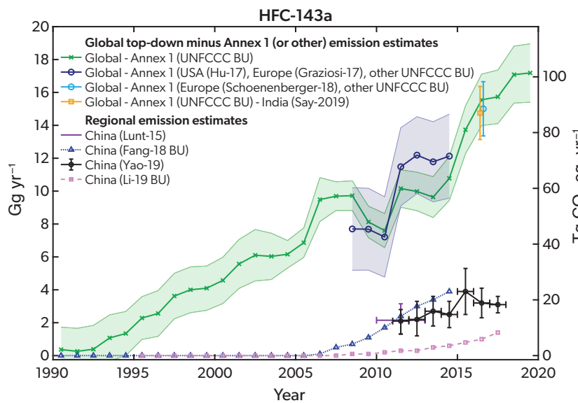
Figure 2-8. As in Figure 2-3, but for HFC-143a.
