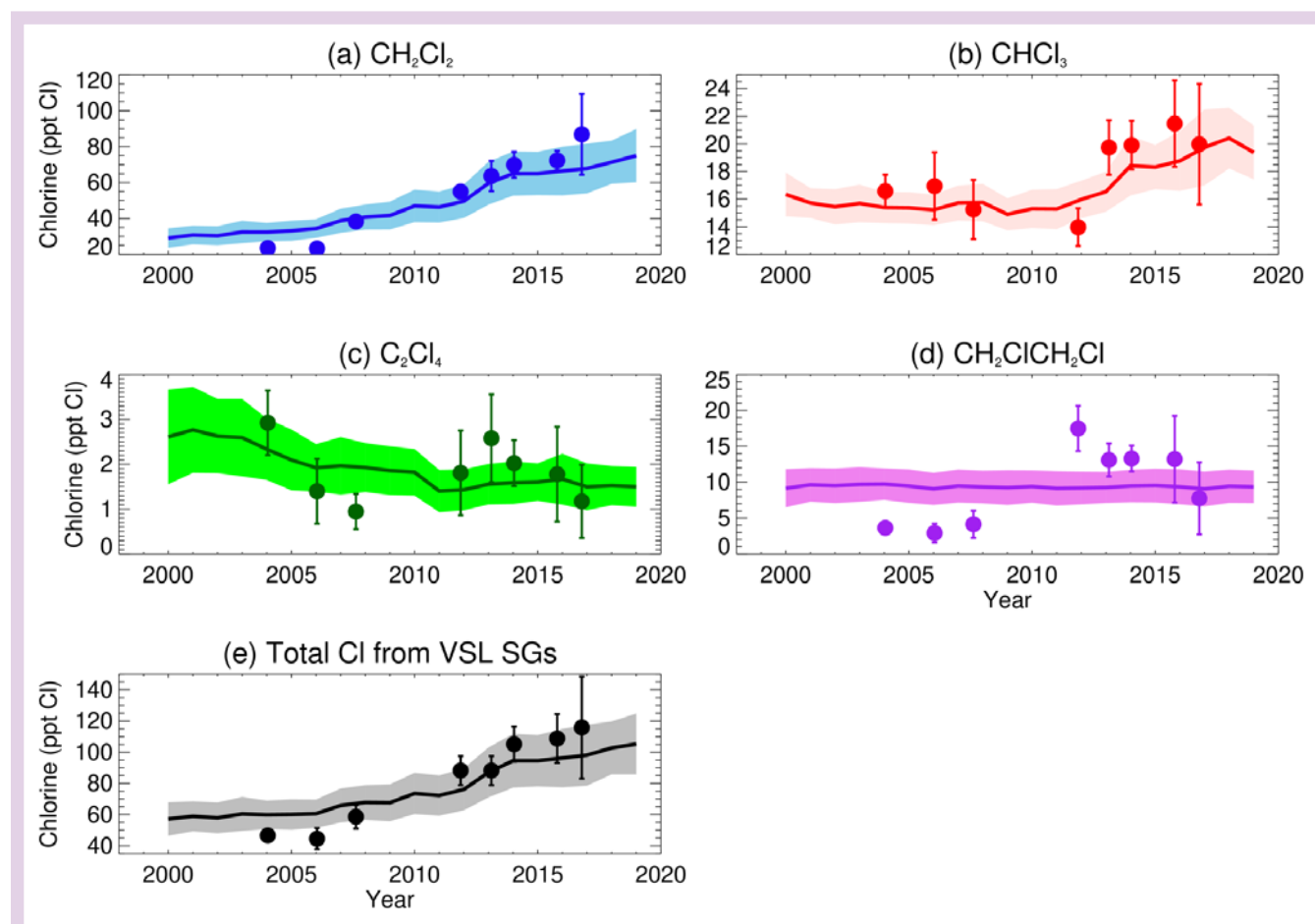
Figure 1-8. Stratospheric chlorine source gas injection (ppt Cl) from (a) CH_2Cl_2 , (b) CHCl_3 , (c) C_2Cl_4 , (d) CH_2CICH_2Cl , and (e) total. Model results (solid lines) with the \pm 1 -sigma uncertainty (shading) are tropical mean ( 20^\circ N – 20^\circ S ) values derived from simulations with the offline 3-D chemistry-transport model TOMCAT/SLIMCAT constrained by observed surface abundances of these source gases. Observed tropopause quantities (filled circles) are averages (vertical bars denote \pm 1 -sigma) for available aircraft data between 16.5 and 17.5 km in the tropics from Pre-AVE in 2004; CR-AVE in 2006; TC4 in 2007; ATTREX in 2011, 2013, and 2014; VIRGAS in 2015; and POSIDON in 2016 (campaign acronyms are provided in Table 1-5). [Updated from Hossaini et al., 2019.]
