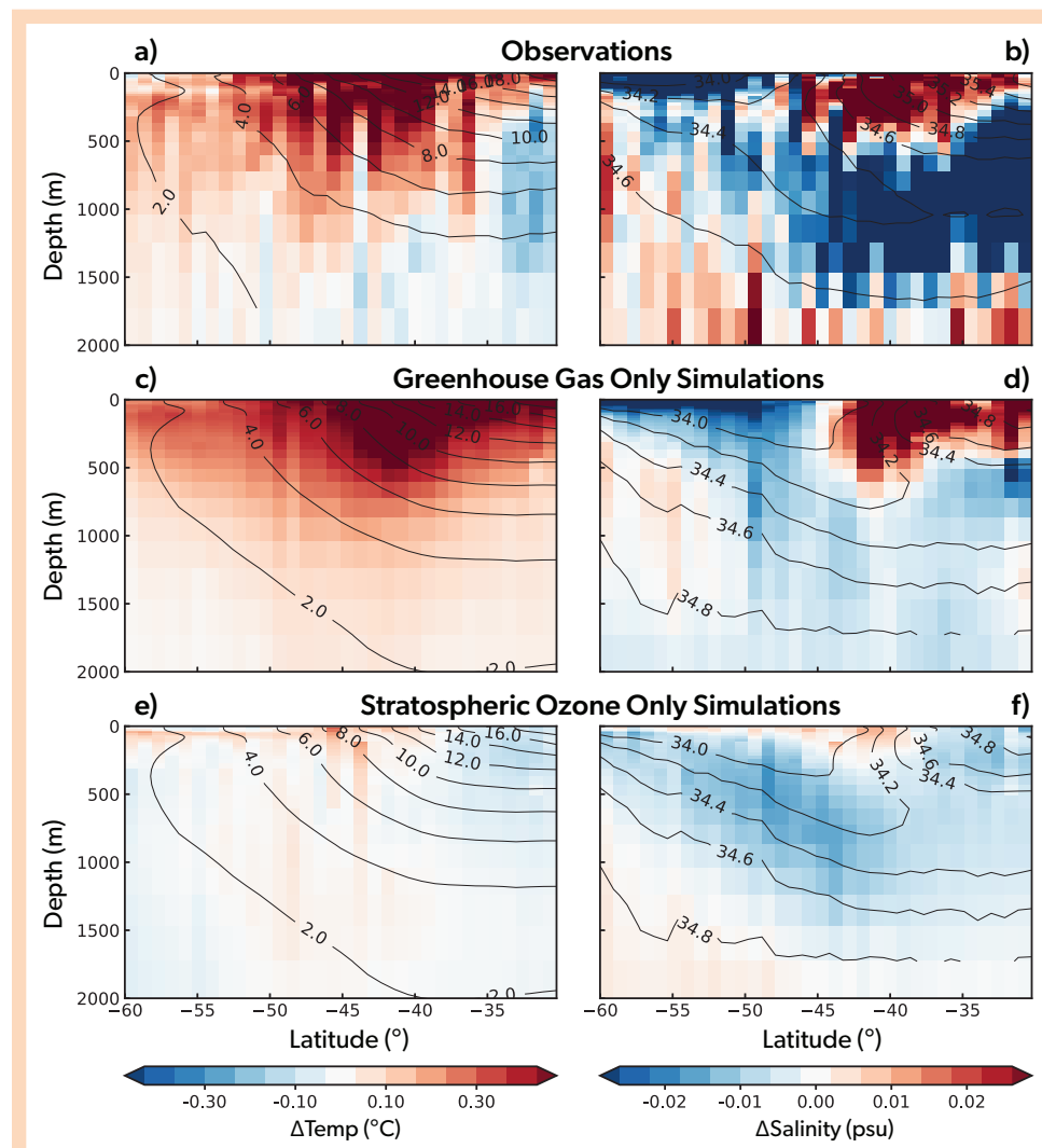
Figure 5-16. Observed and simulated changes in Southern Ocean temperature and salinity. Zonal mean (a, c, e) temperature, and (b, d, f) salinity, from (a, b) observations, (c, d) ensemble means of the CanESM2 greenhouse-gas-only simulations, and (e, f) stratospheric-ozone-only simulations. Anomalies represent the difference between the 2006–2015 mean and the mean over a 1950–1980 base period. Black contours show the climatological temperature and salinity. The CanESM2 fields (c, d, e, f) are subsampled to match observational coverage and scaled to best match the observations using scaling factors of (c) 0.70, (d) 0.74, (e) 1.77, and (f) 0.70. [Adapted from Swart et al., 2018.]
