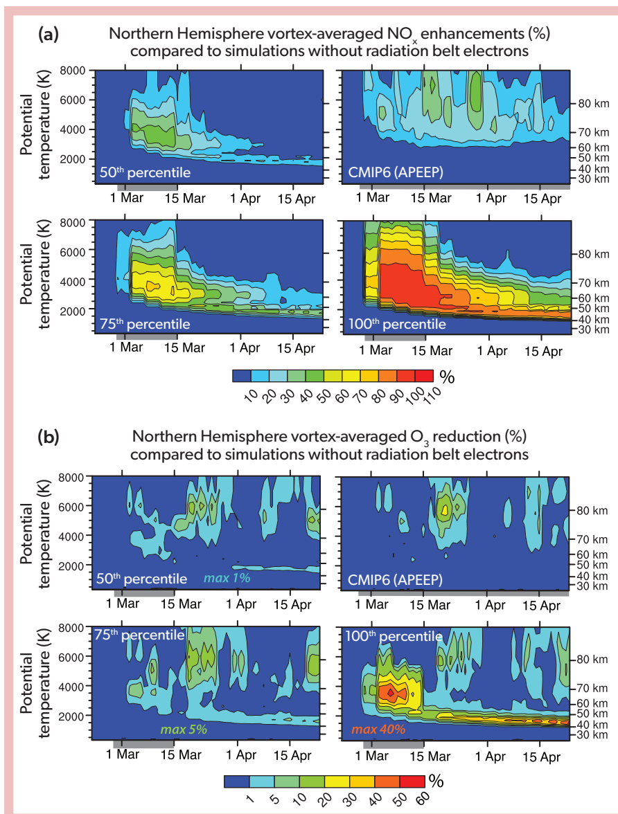
Figure 4-14. WACCM simulations for the March 2013 electron precipitation event showing longer-term (a) enhancements of NO x and (b) reductions of O 3 averaged over the Northern Hemisphere polar vortex from radiation belt electrons. Gray bars along the x-axis represent times when medium energy electron ionization is included in the simulations. Percentiles refer to the flux ratios of the two instruments. [From Duderstadt et al., 2021.]
