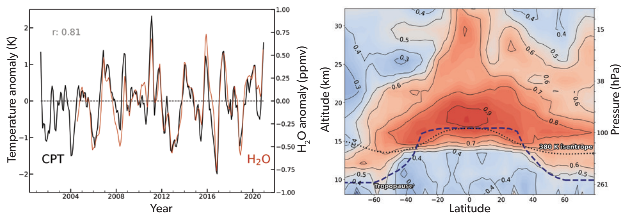
Figure 5-3. Temperature control of water vapor entry at the tropical tropopause. (left) Time series of deseasonalized anomalies in tropical cold point tropopause (CPT) temperature from GPS radio occultation (10°S–10°N) and equatorial (5°N–5°S) 83 hPa water vapor from Aura MLS. (right) Correlation of deseasonalized anomalies in Aura MLS water vapor over 2004–2020 versus water vapor reconstructed from lagged regressions onto the tropical CPT. [Updated from Randel and Park (2019) using MLS v5.1 H 2 O retrievals (Lambert et al., 2020).]
