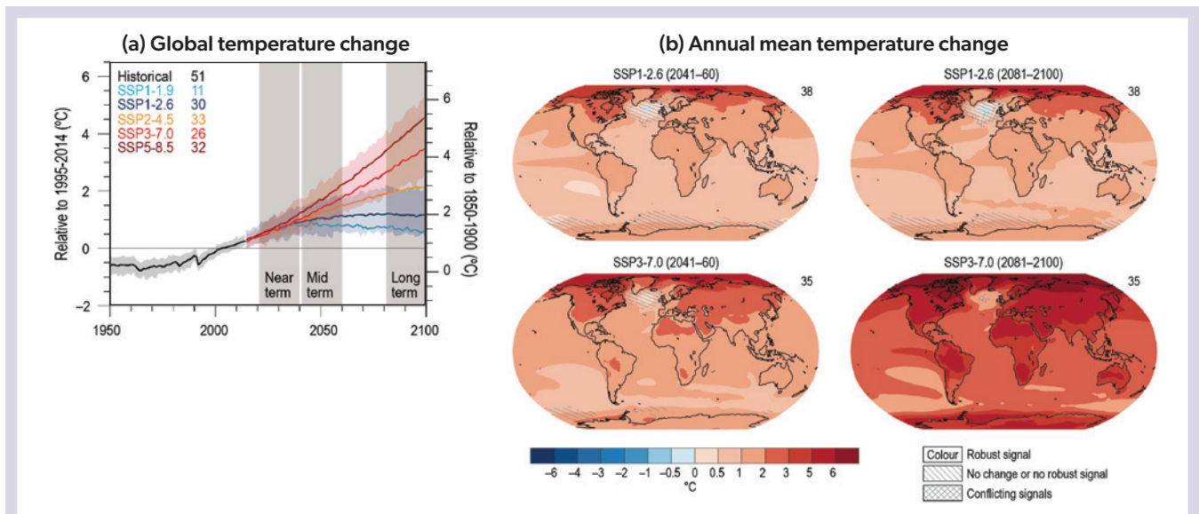
Figure 6-1. (a) Multi-model simulated time series from 1950 to 2100 for global annual average surface air temperature changes relative to the 1995–2014 average (left axis) and the 1850–1900 average (right axis). The curves show averages over the CMIP6 simulations, the shadings around the SSP1-2.6 and SSP3-7.0 curves show 5–95% ranges, and the numbers in the legend after each experiment show the number of model simulations used. (b) The global mean distribution of mid-term (2041–2060) and long-term (2081–2100) changes in annual mean surface temperature. The number of model simulations used is indicated in the top right of the maps. No overlay indicates regions where the change is robust and emerges from internal variability (i.e., 66% of the models show a change greater than the internal-variability threshold, and at least 80% of the models agree on the sign of change). Diagonal lines indicate regions with no change or no robust significant change. Crossed lines indicate areas of conflicting signals. [Both panels reproduced from Lee et al., 2021.]
