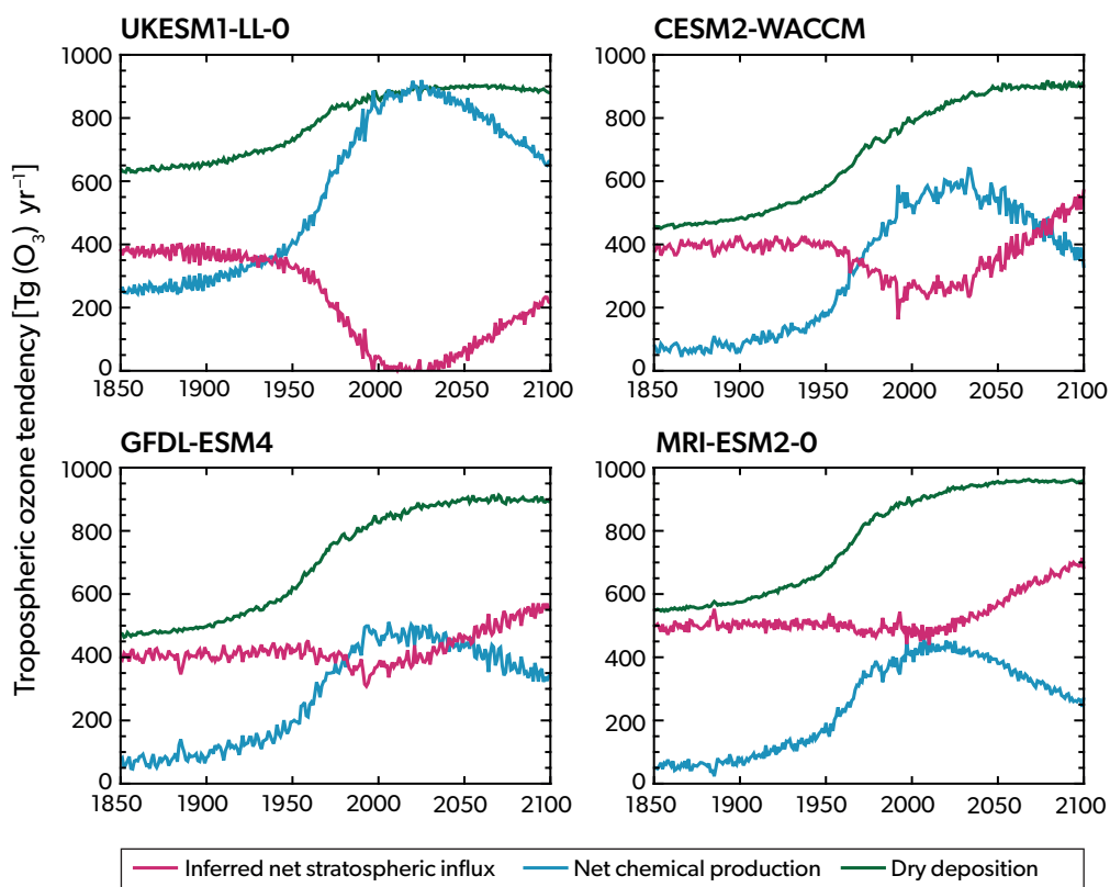
Figure 3-29. Time series of the simulated tropospheric ozone budget terms over 1850–2100 in four CMIP6 models from the historical (1850–2014) and SSP3-7.0 (2015–2100) simulations, showing dry deposition (green), net chemical production (NCP, blue), and the residual (dry deposition minus NCP, assumed to be net stratospheric influx; red). The troposphere is delimited using the WMO tropopause definition. The budget terms are shown for the four CMIP6 models with the required output: UKESM1-0-LL, CESM2-WACCM, GFDL-ESM4, and MRI-ESM2-0. [Adapted from Griffiths et al., 2021.]
