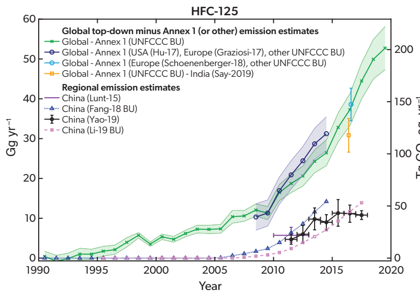
Figure 2-7. As in Figure 2-3, but for HFC-125.
