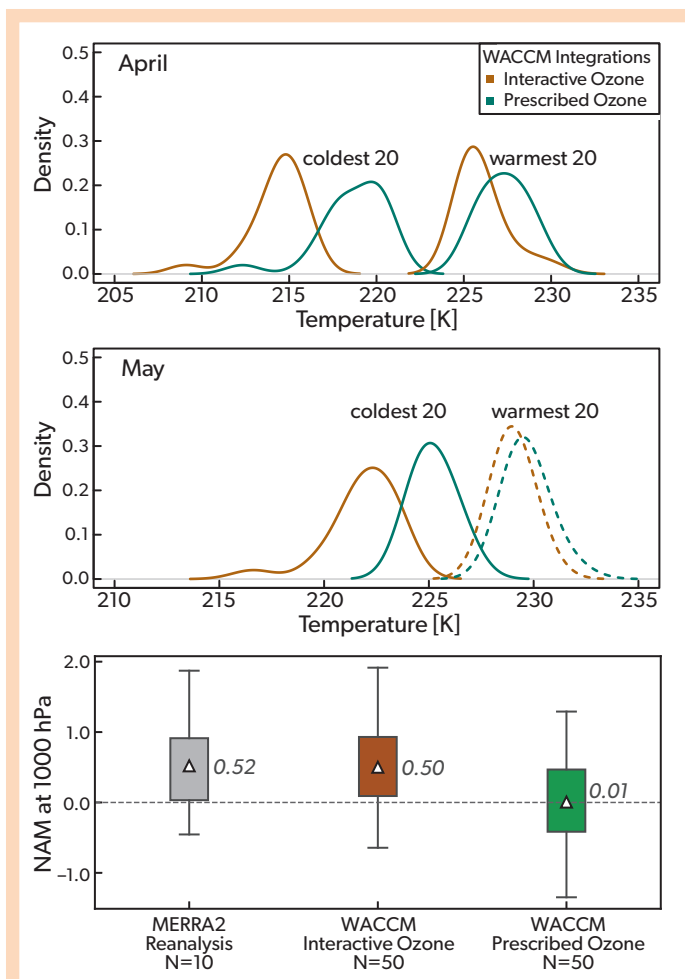
Figure 5-12. Impact of interannual Arctic ozone variations on stratospheric temperatures and tropospheric circulation. Probability distribution functions for (top) April and (middle) May monthly mean Arctic lower stratospheric (50 hPa) polar cap temperature for the coldest and warmest 20 years in perpetual year-2000 Whole Atmosphere Community Climate Model (WACCM) integrations with interactive chemistry (brown) and with prescribed climatological zonal mean ozone (green). Solid curves indicate a significant difference between the two integrations at the 95% level, while dashed curves indicate no significant difference. (bottom) Box plots of the Northern Annular Mode (NAM) index at 1000 hPa following winters with extreme ozone loss. The box plot shows the distribution of the mean NAM Index (20 - 90°N) at 1000 hPa in the month following the ozone minimum for the MERRA2 reanalysis (gray), WACCM integrations with interactive middle atmosphere chemistry (brown) and the WACCM integrations in which ozone chemistry is decoupled from the radiation scheme, i.e. the radiation scheme uses a prescribed climatological year-2000 zonal mean ozone field (green). In the bottom panel, in the WACCM integrations with prescribed ozone, chemistry is still calculated in the background so that ozone depletion events can be identified following the methodology in Friedel et al. (2022). Triangles and numbers indicate the mean NAM index in the month after the ozone minima, averaged over the 25% most extreme winters. The upper and lower edges of the boxes show the upper and lower quartile, the whiskers represent the maximum and minimum values of the respective distribution. [Top and middle panels adapted from Rieder et al., 2019, and bottom panel adapted from Friedel et al., 2022.]
