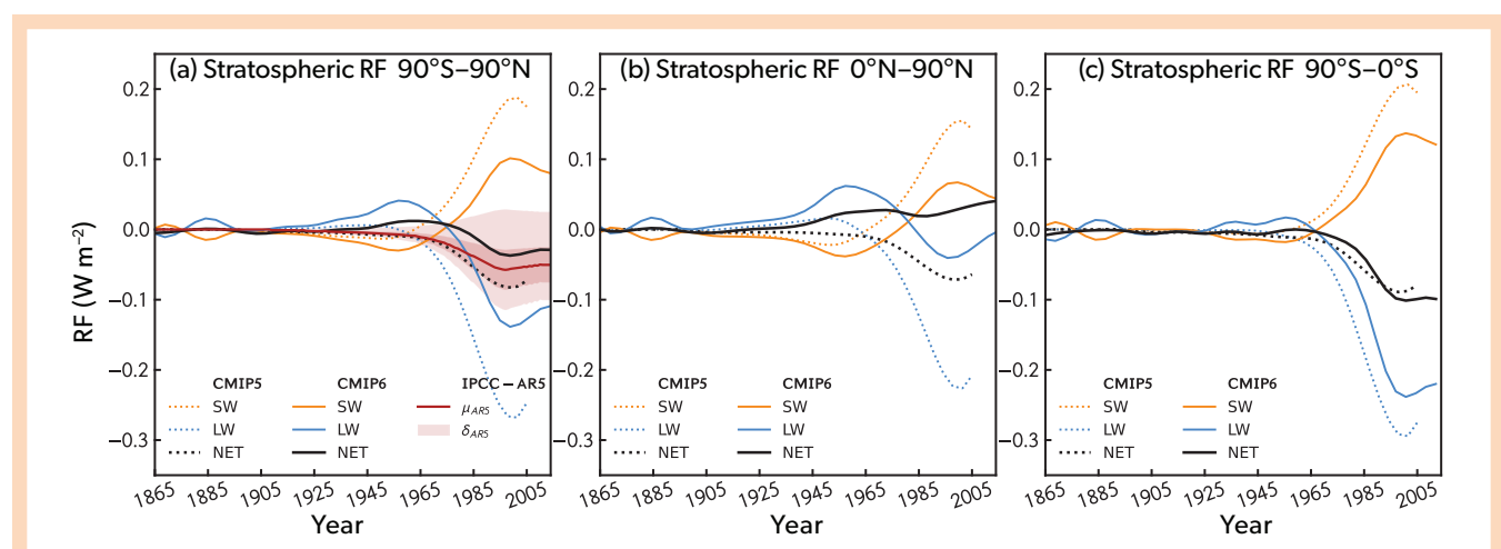
Figure 5-8. Radiative forcing from stratospheric ozone relative to 1850 and its evolution over the 20 th century, from the ozone datasets compiled for CMIP6 (solid lines) and CMIP5 (Ciannoni et al., 2011; dotted lines), as well as the IPCC AR5 estimate (red line) and its uncertainty (shading), for the global mean ( left panel ), Northern Hemisphere ( center panel ), and Southern Hemisphere ( right panel ). The stratosphere-adjusted RF in this figure is evaluated at the tropopause. Yellow lines denote the SW forcing, while blue lines show the LW component in the CMIP5 and CMIP6 estimates. [Adapted from Checa-Garcia et al., 2018.]
