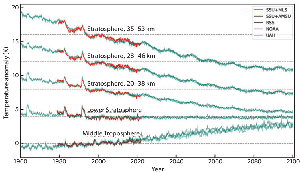
Figure 5-1. Time series of global average temperature anomalies for broad-layer averages from the middle troposphere to the upper stratosphere (bottom to top). Satellite observations are shown for 1979–2020 (see legend), updated from data described in Steiner et al (2020). Note that results from the different observational data sets often overlap, highlighting broad-scale agreement. Temperature anomalies are also shown for WACCM model simulations (green colors) for the recent past (1960–2018), from the so-called Ref-D1 CCMI-2022 simulations incorporating known historical forcings, and including 4 separate realizations. Simulations for 2015–2100 follow the Ref-D2 CCMI-2022 specifications, using SSP2-4.5 forcing and WMO2018 A1 halogens; the runs include an interactive ocean, and 3 realizations are shown. Anomalies from the two sets of model runs are merged for the overlap period 2015–2018.
