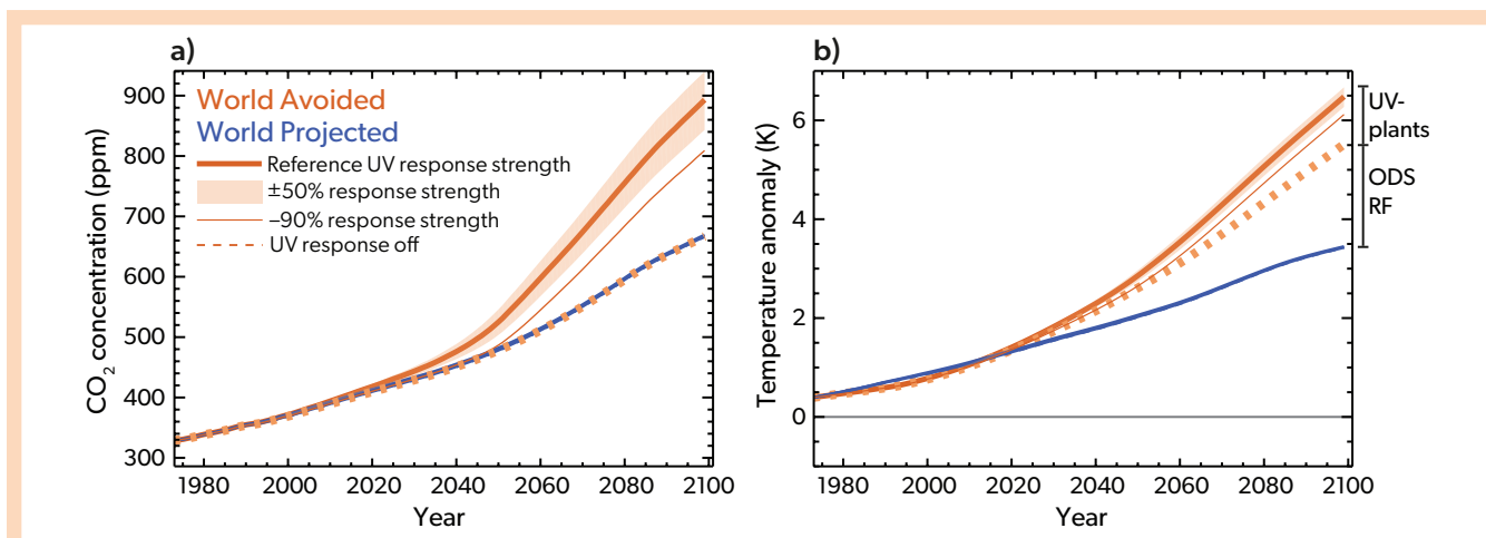
Figure 5-19. The effect of UV-driven changes in vegetation (UV-plants) on atmospheric CO 2 and surface temperature. (a) Time series of atmospheric CO 2 concentrations and (b) anomalies in global-mean surface air temperature for a regular future projection (World Projected, blue; approximately RCP6.0) and a World Avoided projection (World Avoided, orange), estimated using a carbon cycle model. The dashed orange lines are results from a World Avoided projection with the ‘UV response off’, the shading around the thick orange lines indicates the range of the responses from the simulations with 50% and 150% UV response strength (with respect to the reference UV case) and the thin orange lines show the effect of reducing the UV response strength to -90%. The labelled ranges in (b) indicate the World Avoided warming above the World Projected that results from direct radiative forcing of the additional CFCs and the additional CO 2 from the UV-driven damage to plants and their ability to act as a carbon store. [Adapted from Young et al., 2021.]
