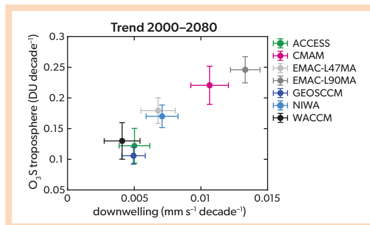
Figure 5-6. Relationship between downwelling changes and stratosphere-to-troposphere ozone transport, shown as a scatter plot of trends in a stratospheric ozone tracer integrated over the troposphere versus extratropical downwelling acceleration in the lower stratosphere (averaged 30°N/30°S and the poles at 70 hPa) for seven models, based on CCM1-1 REF-C2 simulations. The stratospheric ozone tracer is the ozone that originated in the stratosphere and has chemical and depositional loss (but no production) in the troposphere. [Adapted from Abalos et al., 2020.]
