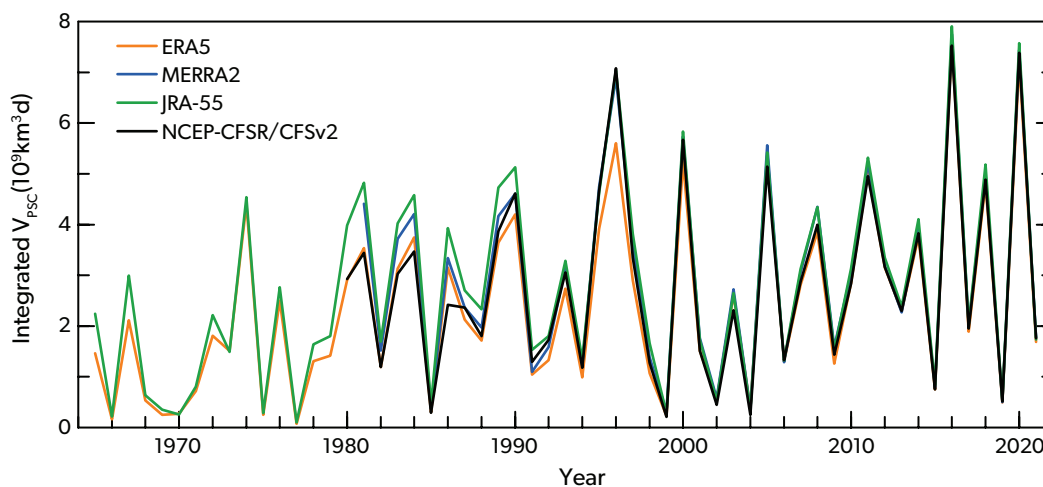
Figure 4-2. The Arctic time-integrated PSC volume, V_{\text{PSC}} , calculated using the method of Rex et al. (2006) for the four indicated reanalysis products. The V_{\text{PSC}} values are integrated from 1 November until 30 April for each Arctic PSC season. The ERA5 result is a combination of ERA5-BE (preliminary version, prior to 1979), ERA5, and ERA5.1 (2000–2006). [Updated from Figure 4-2 in Langematz, Tully et al., 2018.]
