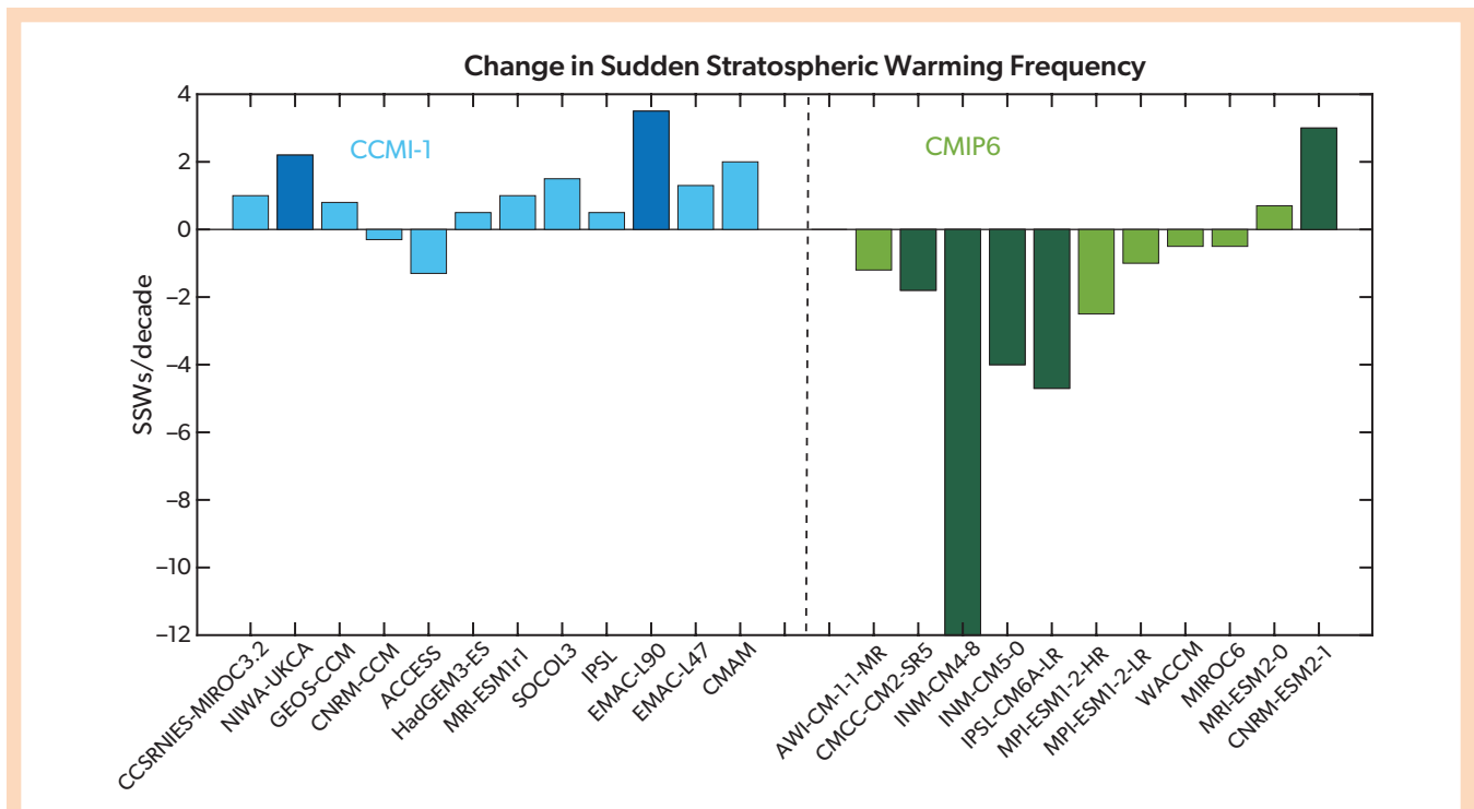
Figure 5-7. Simulated change in the frequency of NH Sudden Stratospheric Warming (SSW) events in the future (2061–2100) relative to the 1960–1999 average in CCMI-1 model simulations (REF-C2; blue bars) and in CMIP6 model simulations under scenario SSP3-7.0 (green bars). The SSW definition is based on the reversal of the zonal-mean zonal wind at 60°N and 10 hPa to easterlies (see Charlton and Polvani, 2007, for the exact definition). Darker colored bars in both indicate statistically significant future-minus-past differences at the 95% confidence level. [Updated from Ayarzagüena et al., 2018.]
