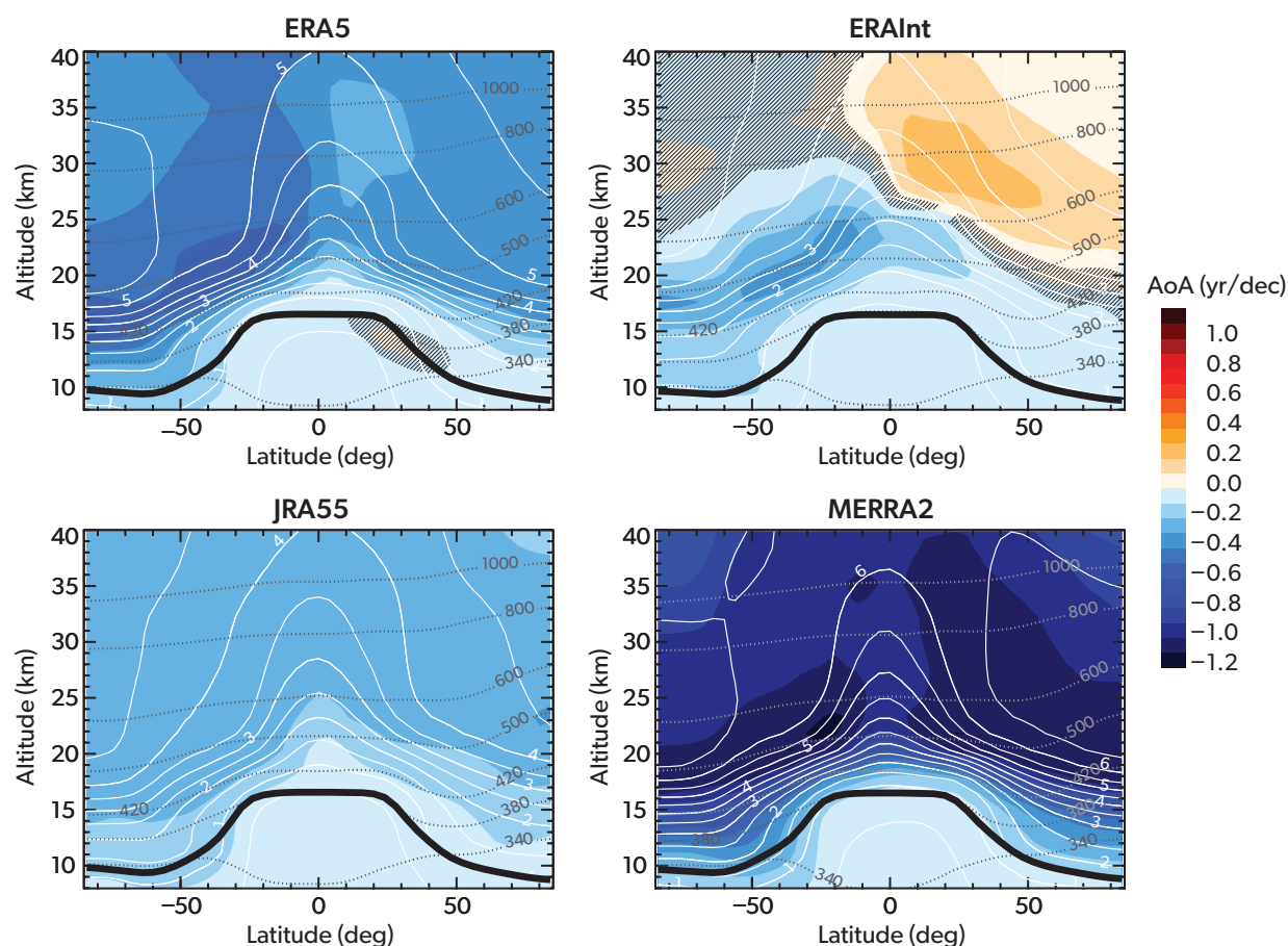
Figure 5-5. Trends in mean AoA in four modern reanalyses over the period 1989–2015 (shading), computed using the Lagrangian transport model CLaMS. Thin solid contours show the mean AoA climatology, with contour spacing of six months. The solid thick contour shows the lapse-rate WMO tropopause. Thin dashed contours show selected isentropes with labeled values in K. Note that the updated ERA5.1 is used for the 2000–2006 period in the ERA5 panel, as in Ploeger et al. (2021). [Adapted from Ploeger et al., 2019, 2021.]
