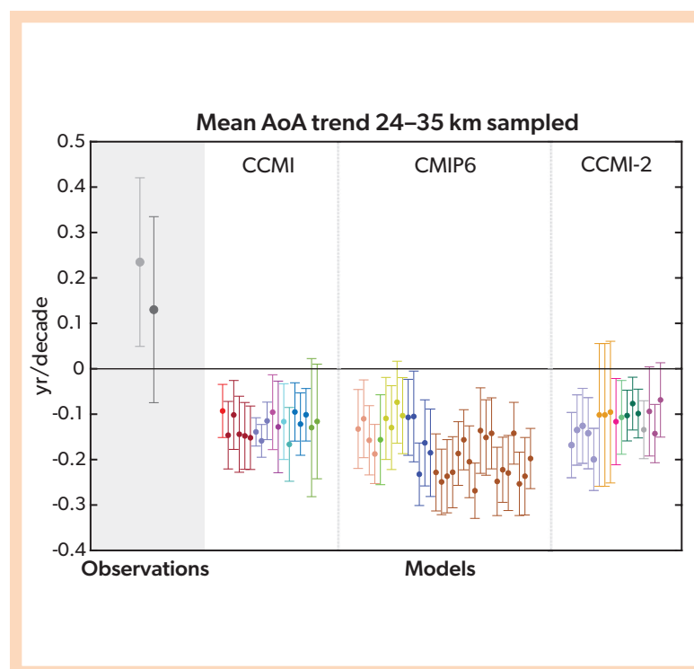
Figure 5-4. Mean AoA trends for the period 1975–2005 from observations and model simulations, with model data sampled at times and locations corresponding to the observations (Engel et al., 2009; Fritsch et al., 2020). Specifically, AoA is averaged over 24–35 km log-pressure altitudes and sampled at the same latitudes and months as the observations. Three families of model simulations are shown: CCM1 REF-C1, CMIP6 historical, and CCM12 REF-D1. Each model is represented in a different color, and multiple ensemble simulations are included for some models, to account for the influence of internal variability on the trends. The mean AoA trend derived from observations is shown on the left (inside the gray shaded area): the original value from Engel et al. (2009) (light gray), and that obtained from the same data but using an updated method to derive AoA from tracer concentrations, as described in Fritsch et al. (2020) (dark gray). Error bars represent least square regression slope uncertainty at the 95% confidence level for the models, while for the observations they include additional measurement error estimates. [Adapted from Abalos et al., 2021.]
