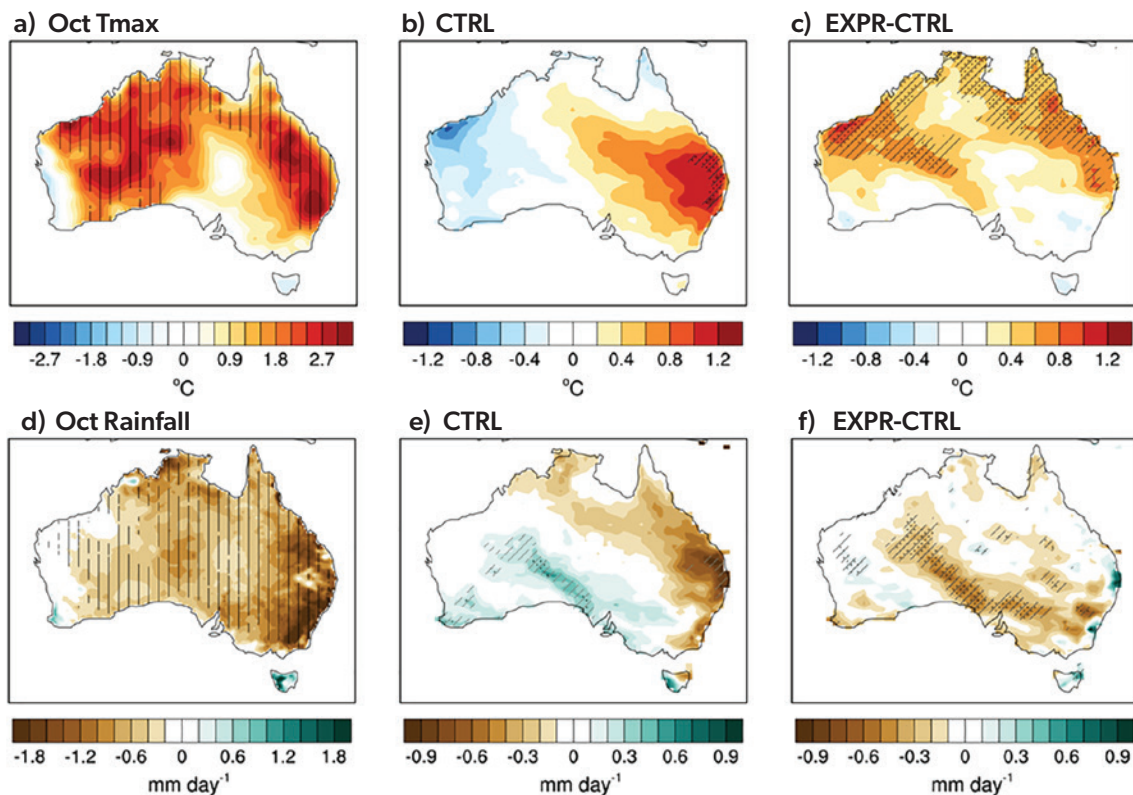
Figure 5-11. Effect of stratospheric ozone anomalies on surface climate in October 2002. Panels (a) and (d) show the observed anomaly in (a) maximum temperature (units: K) and (d) precipitation (units: mm/day) for October 2002. Panels (b) and (e) show the simulated temperature (b) and precipitation (d) anomalies, averaged across and 11 members ensemble of model simulations using the ACCESS forecasting model when fixed climatological ozone concentrations are used (CTRL). Panels (c) and (f) show the ensemble-mean difference in temperature (c) and precipitation (f) between model simulations where the observed 2002 ozone anomalies were used (EXPR) and the CTRL simulations (shown in panels b and d) using a fixed climatological ozone (CTRL). Hatching in (a) and (d) indicates where the October 2002 anomaly falls in the upper 20% and lower 20% tails, respectively, of the observed distribution for the period 1990–2012 (excluding 2002). Stippling and hatching in (b) and (e) indicate where the predicted values fall within the 5% and 10% tails, respectively, of the distribution based on the hindcast control simulations spanning the period 1990–2012 (excluding 2002). Stippling and hatching in (c) and (f) indicate where the null hypothesis of no difference between EXPR and CTRL is rejected at the 5% (10%) level based on resampling of the 11 ensemble members from the CTRL and EXPR for 2002. [Adapted from Hendon et al., 2020.]
