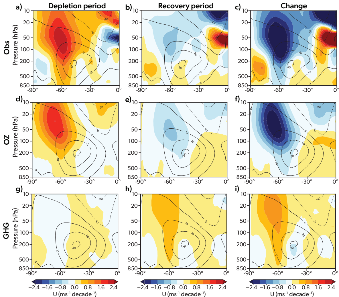
Figure 5-18. Observed and simulated Southern Hemisphere zonal average zonal wind trends. The top row shows an average of four reanalysis data products (ERA-Interim, JRA-55, MERRA2-ana, MERRA2-asm), and the middle and bottom rows show an ensemble mean of CCMVal-2 and CCM1 chemistry-climate model integrations. Latitude-altitude cross sections of zonal average zonal wind trends (color shading) for DJF are shown for the depletion period ( left column ), recovery period ( middle column ), and the difference between the two ( right column ). Fingerprints are shown for the simulations with single forcings by (d–f) ozone (OZ) and (g–i) GHGs. For illustrative purposes, the contours show the climatologies (in \text{m s}^{-1} ; for d–i, the climatologies are for the ALL-forcing integrations; for f and i, the climatology is over the entire change period). [Adapted from Banerjee et al., 2020.]
