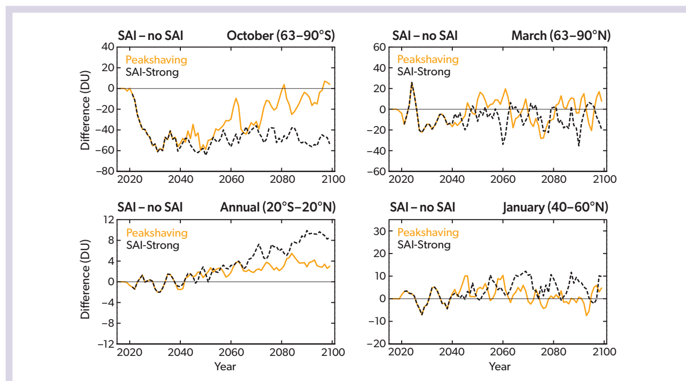
Figure 6-14. Ensemble mean differences in TCO between simulations that include SAI (in the peakshaving [orange] and strong [black] SAI scenarios) and TCO in the baseline simulation (no SAI), for different regions and seasons (different panels), as shown in Figure 6-13. A running mean of three years has been applied to the differences.
