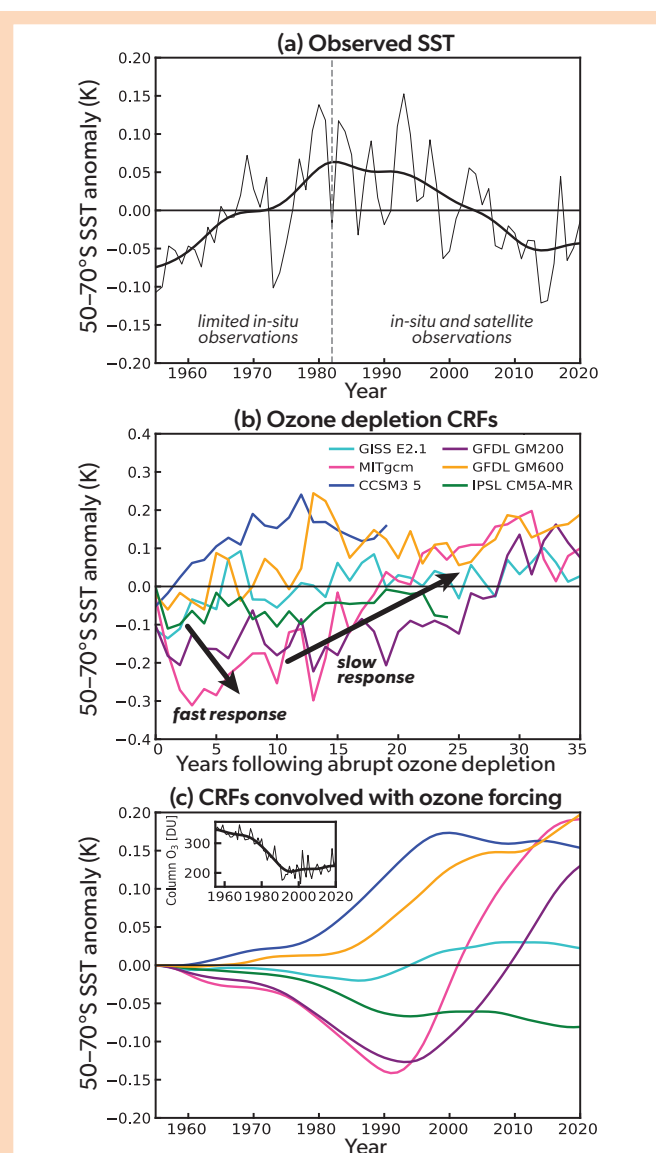
Figure 5-17. Observed and simulated evolution of high-latitude SST. (a) Observed 50–70°S average SST anomaly time series from the HadISST dataset. Anomalies are calculated relative to the 1955–2020 mean, and the bold line shows the 20-year running mean smoothed with a Hanning window. (b) Ensemble-mean time series of annual-mean SST anomaly averaged over 50–70°S from six different climate models simulating the climate response functions (CRFs) to abrupt ozone-hole conditions. The idealized ozone forcing reveals two timescales to the SST response—an initial cooling (the fast response) followed by an eventual warming (the slow response)—as indicated by large arrows; however, there is a large spread in responses across models. (c) Convolution of the anomalous SST response to abrupt ozone-hole conditions in (b) with time-evolving ozone forcing, as shown in the insert (October-mean 60–90°S column ozone from the WACCM chemistry-climate model). The convolved SST time series in (c) differ from the observed SST time series in (a), suggesting ozone depletion is unlikely to have been the primary driver of the observed high-latitude SST cooling since ~1980. [Adapted from Seviour et al., 2019.]
