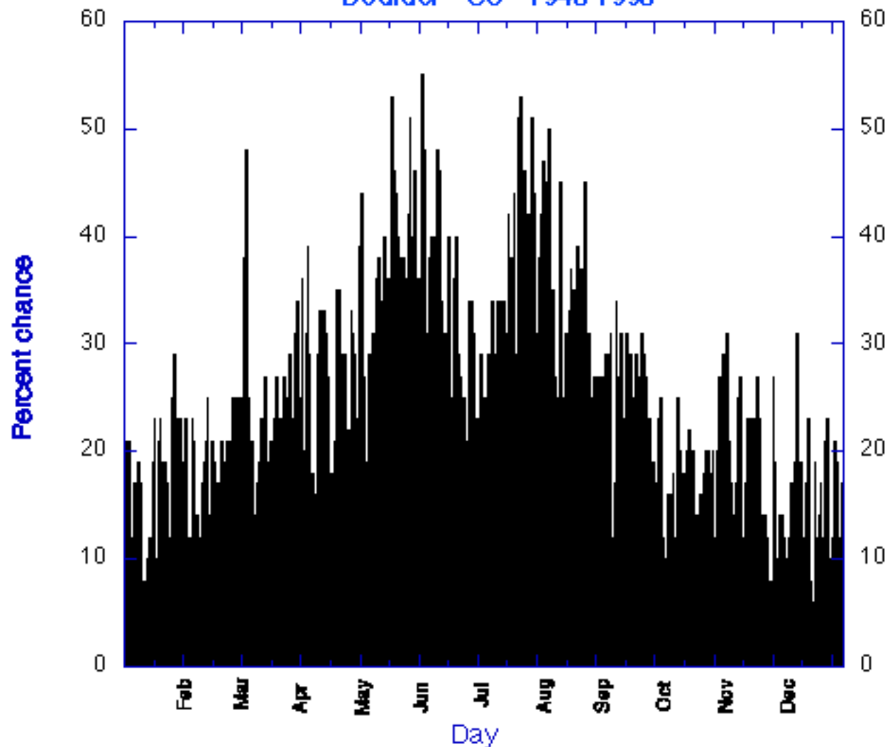
Daily chance of greater than trace precipitation Boulder CO 1948-1998
