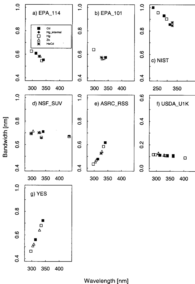
Fig. 5.3. Bandwidth as a function of wavelength for the instruments indicated in each panel from high-resolution spectral scans of the singlet lines from the sources indicated in the legend.
